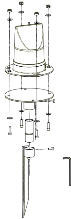
Frangible Stake Mount
