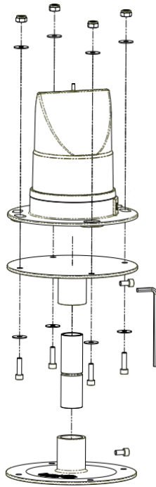
Frangible Concrete Mount
